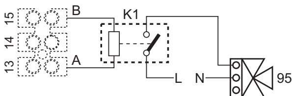
fig. 95- Connection of the 3-way valve with 2 wires
