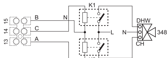
fig. 96- Connection of the 3-way valve with 3 wires
